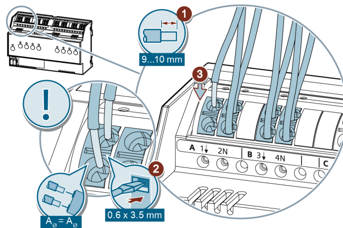
Fig. 4: Example graphic: Binary input 8 x AC/DC 10...230 V
